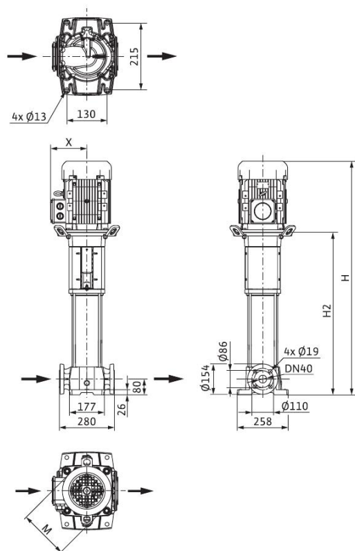
尺寸图 Dimension drawing Helix FIRST V 10, 30 bar
