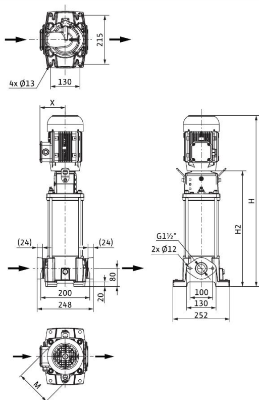
尺寸图 Dimension drawing Helix FIRST V 10, PN 16
