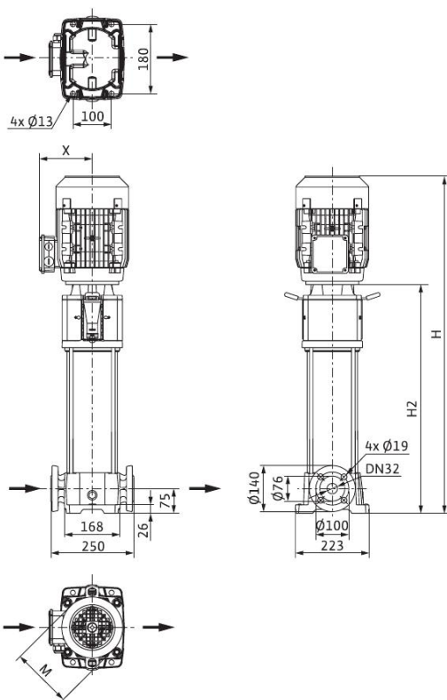
尺寸图 Dimension drawing Helix FIRST V 6, 30 bar
