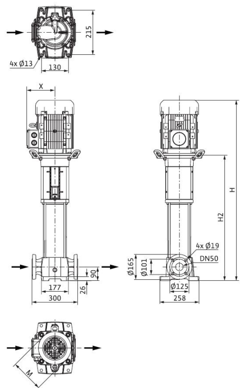
尺寸图 Dimension drawing Helix FIRST V 16, 30 bar
