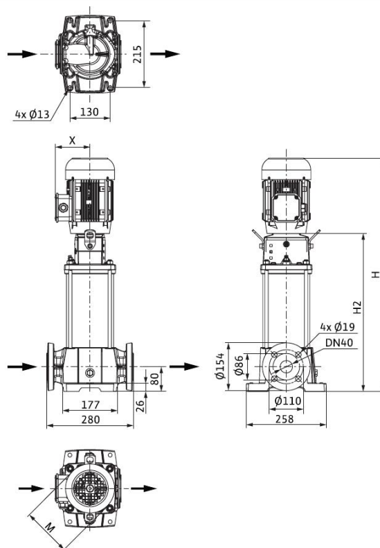
尺寸图 Dimension drawing Helix FIRST V 10, PN 25
