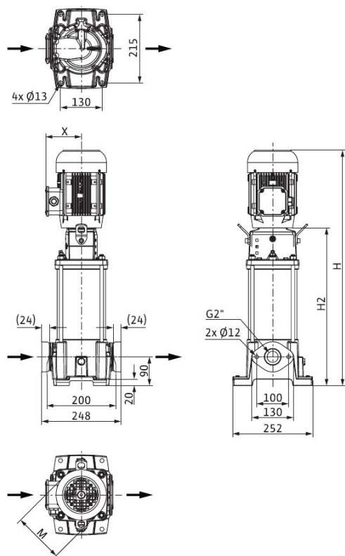
尺寸图 Dimension drawing Helix FIRST V 16, PN 16
