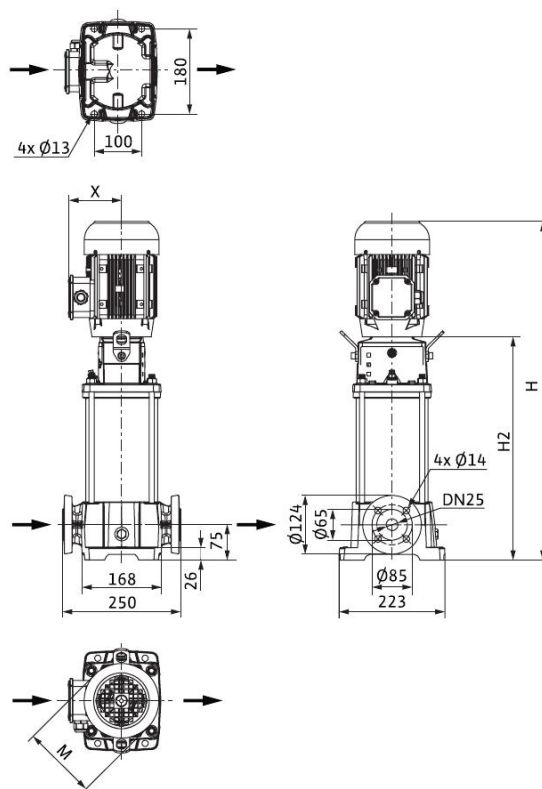
尺寸图 Dimension drawing Helix FIRST V 2-4, PN 25
