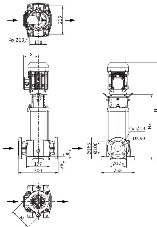
尺寸图 Dimension drawing Helix FIRST V 16, PN 25
