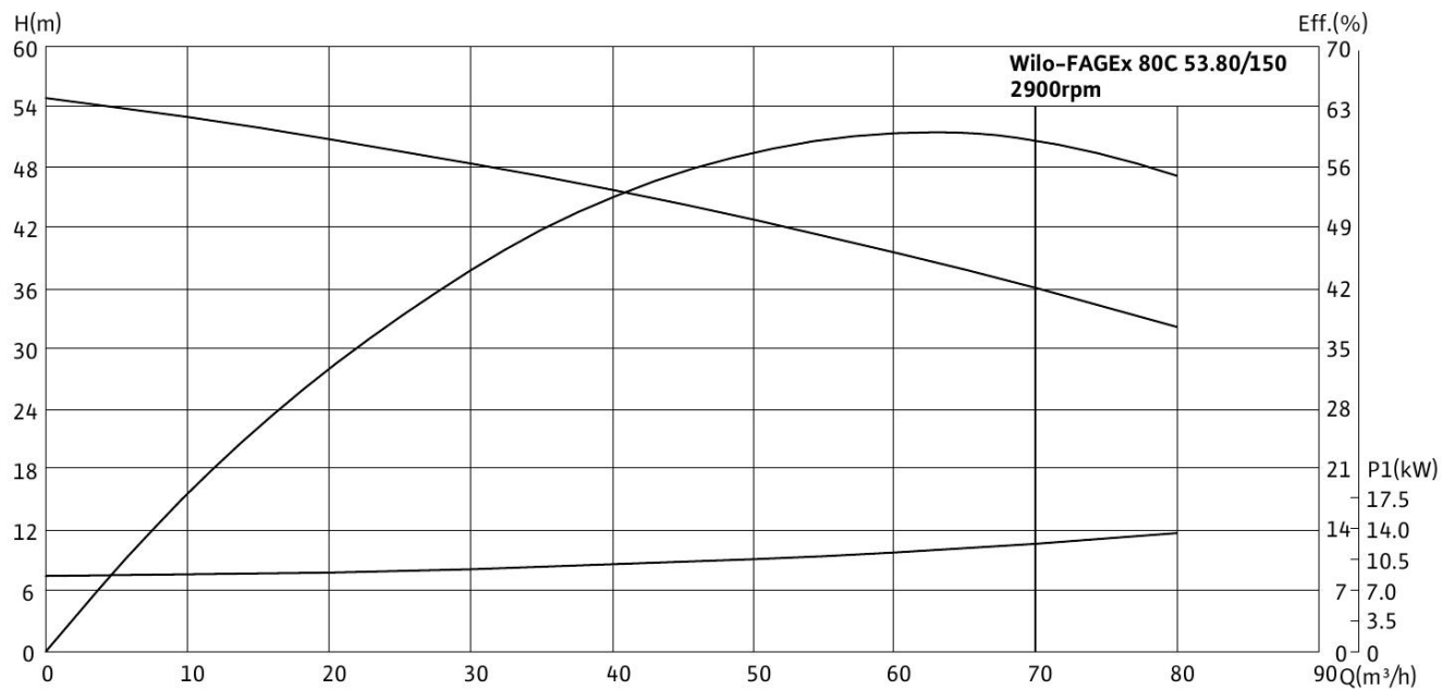
Wilo-FAGEx 80C 53.80/150
