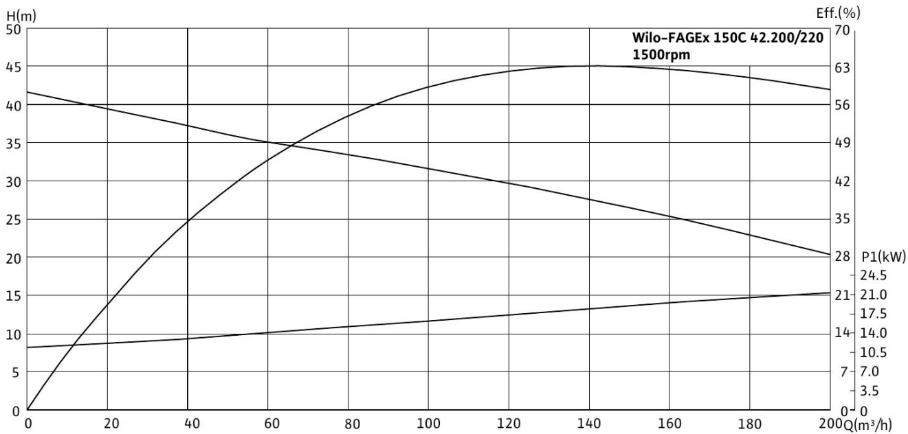
Wilo-FAGEx 150C 42.200/220
