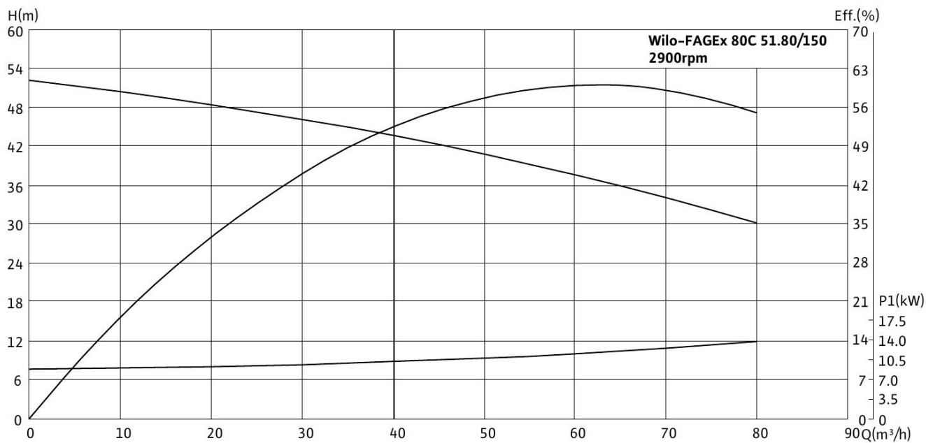
Wilo-FAGEx 80C 51.80/150
