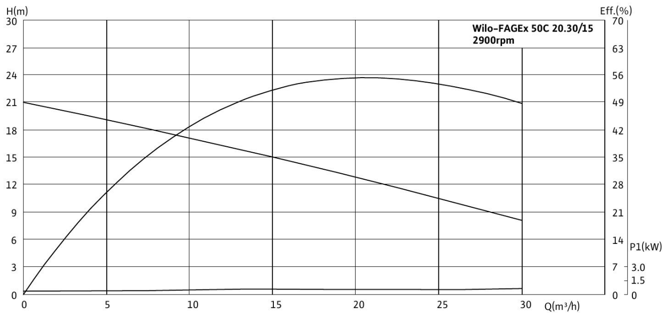
Wilo-FAGEx 50C 20.30/15
