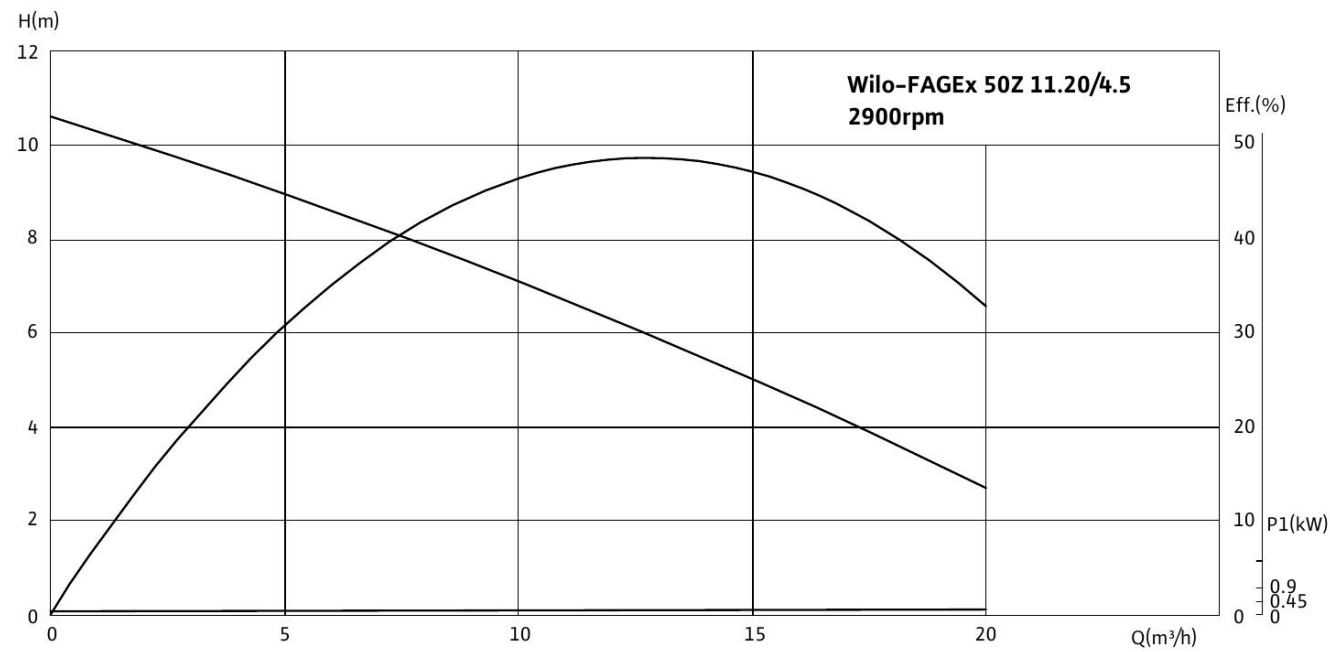
Wilo-FAGEx 50Z 11.20/4.5
