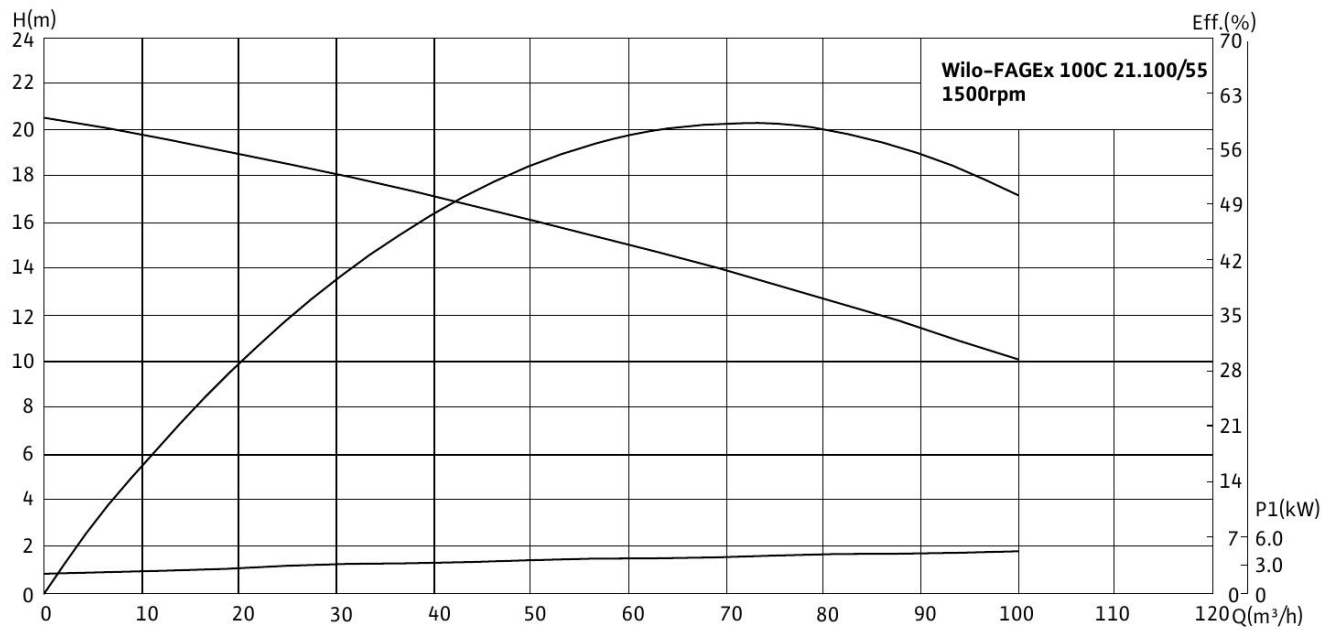
Wilo-FAGEx 100C 21.100/55
