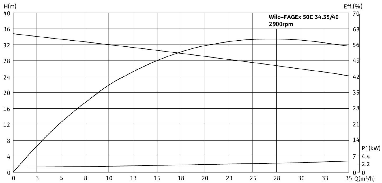
Wilo-FAGEx 50C 34.35/40
