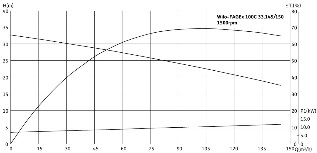
Wilo-FAGEx 100C 33.145/150
