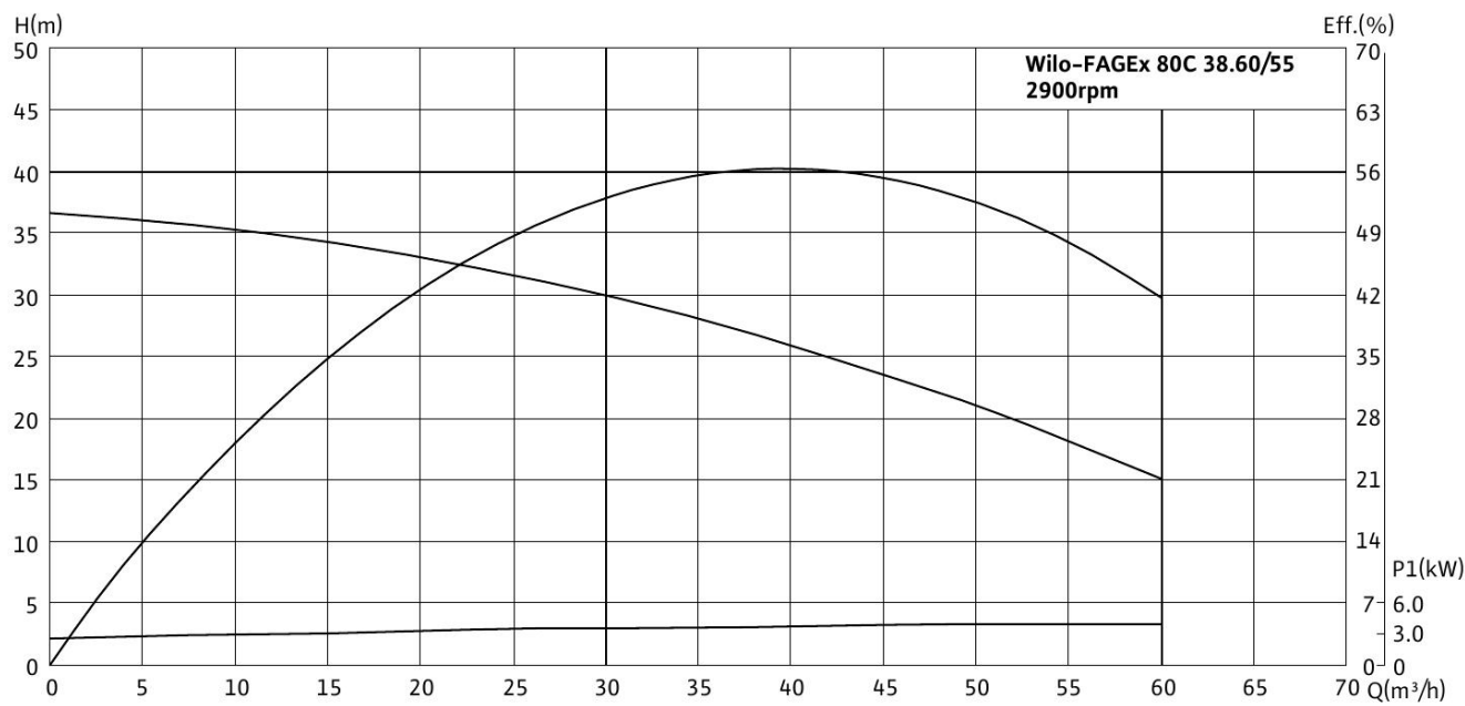
Wilo-FAGEx 80C 38.60/55
