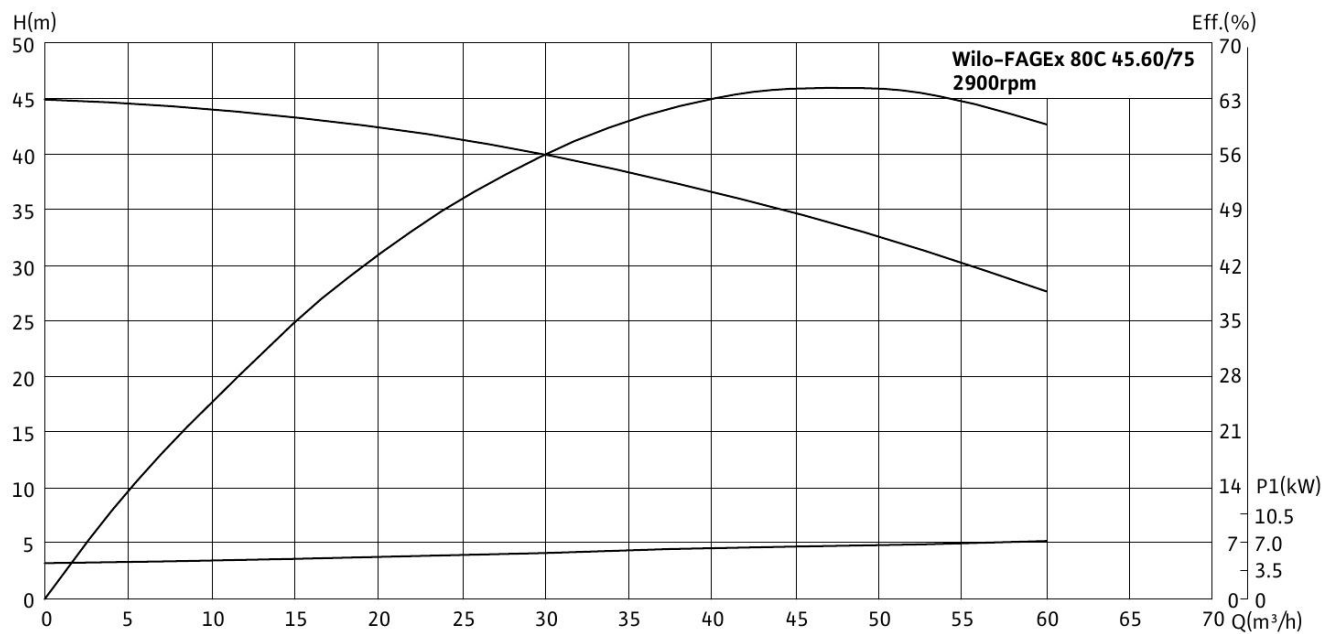
Wilo-FAGEx 80C 45.60/75
