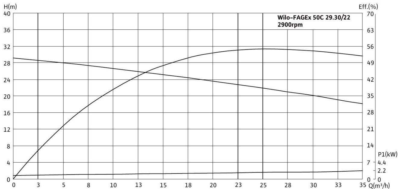
Wilo-FAGEx 50C 29.30/22
