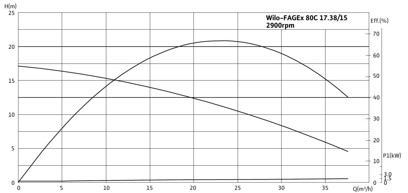
Wilо-FAGEx 80C 17.38/15
