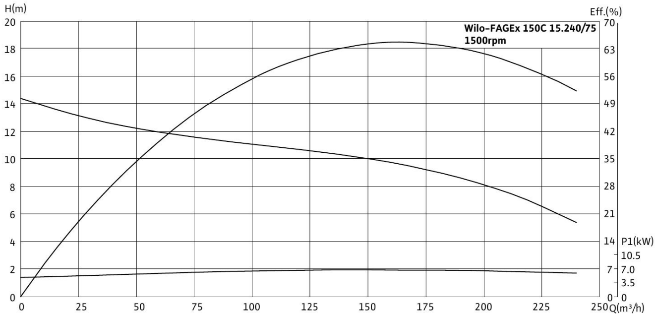
Wilo-FAGEx 150C 16.240/110
