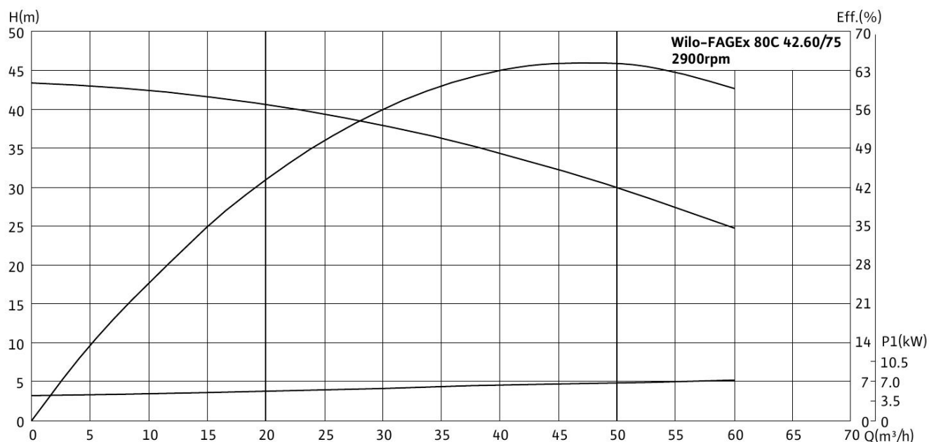
Wilo-FAGEx 80C 42.60/75
