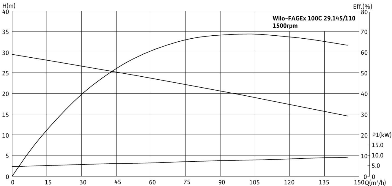
Wilo-FAGEx 100C 29.145/110
