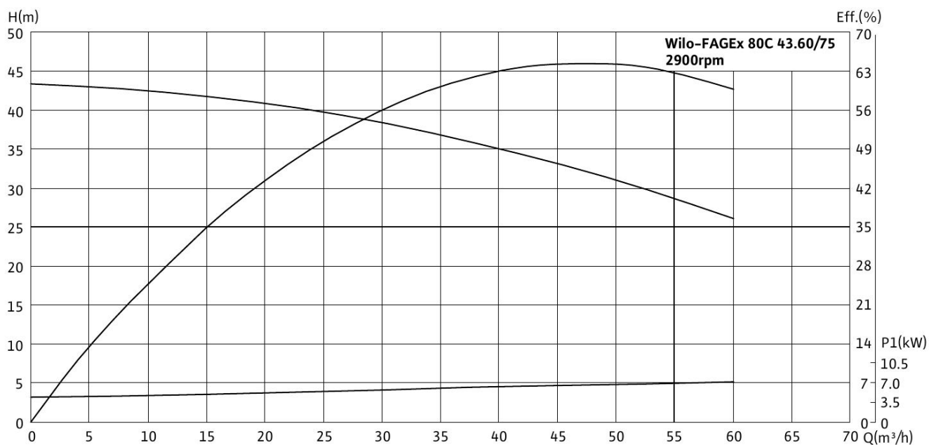
Wilo-FAGEx 80C 43.60/75
