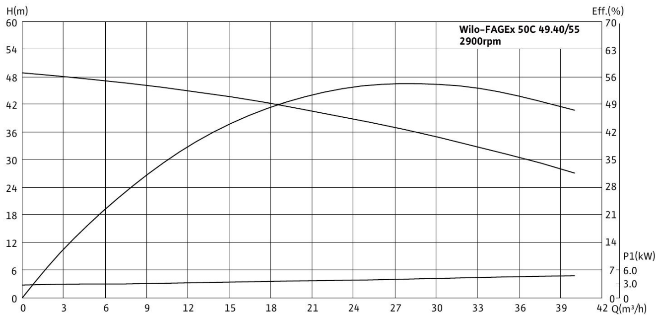
Wilo-FAGEx 50C 49.40/55
