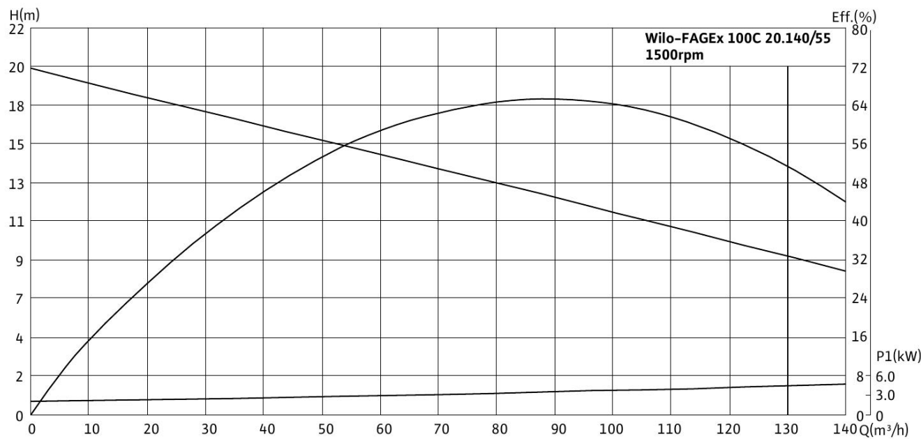
Wilo-FAGEx 100C 20.140/55
