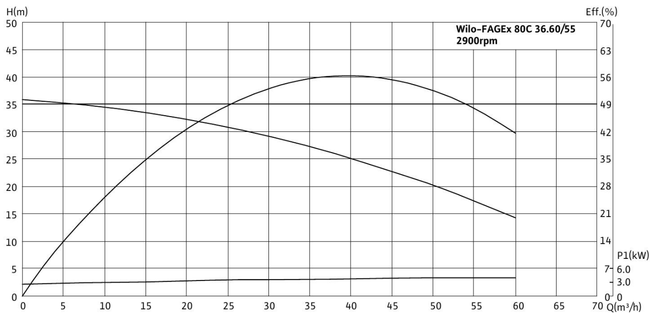
Wilo-FAGEx 80C 36.60/55
