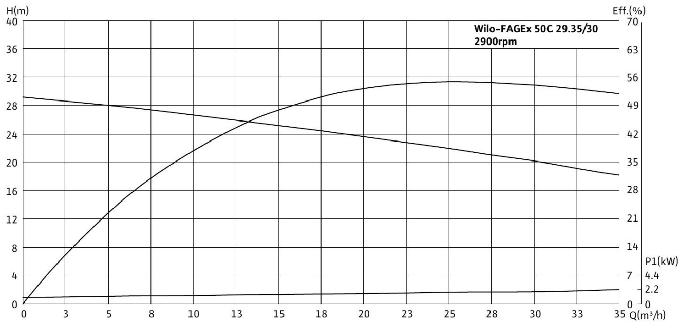
Wilo-FAGEx 50C 29.35/30
