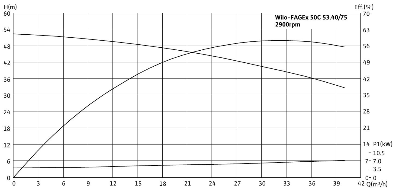
Wilo-FAGEx 50C 53.40/75
