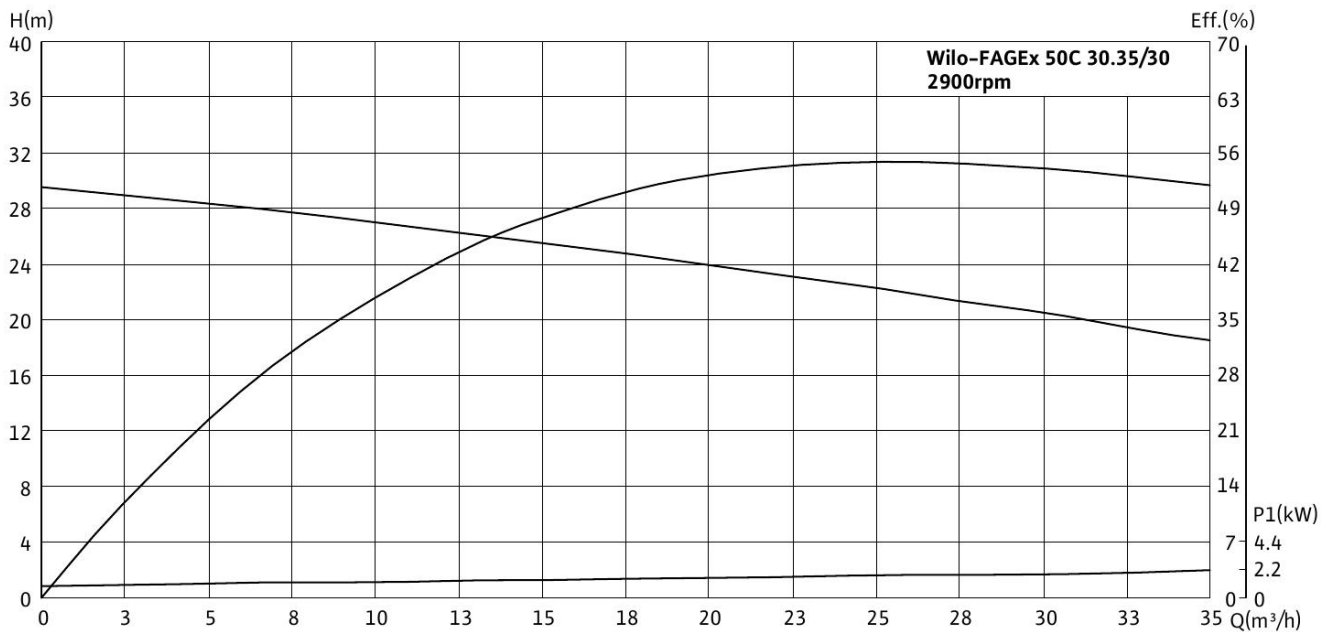
Wilo-FAGEx 50C 30.35/30
