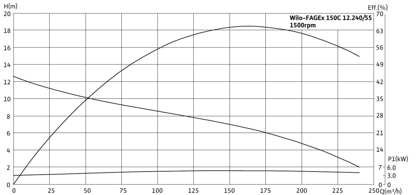
Wilo-FAGEx 150C 12.240/55
