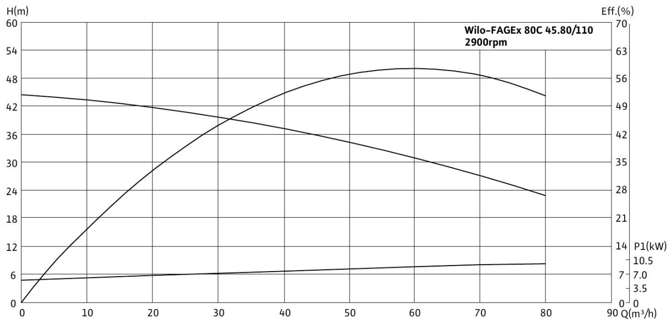
Wilo-FAGEx 80C 45.80/110
