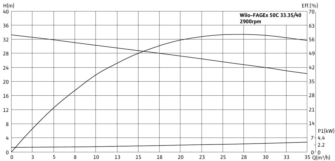
Wilo-FAGEx 50C 33.35/40
