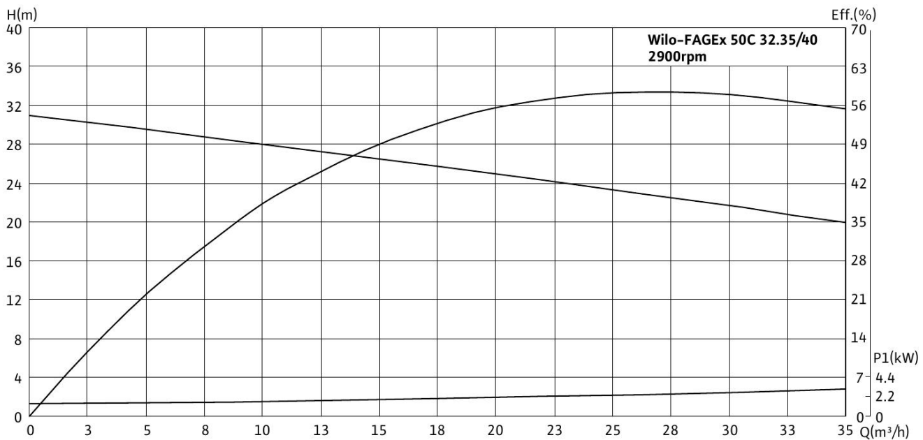
Wilo-FAGEx 50C 32.35/40
