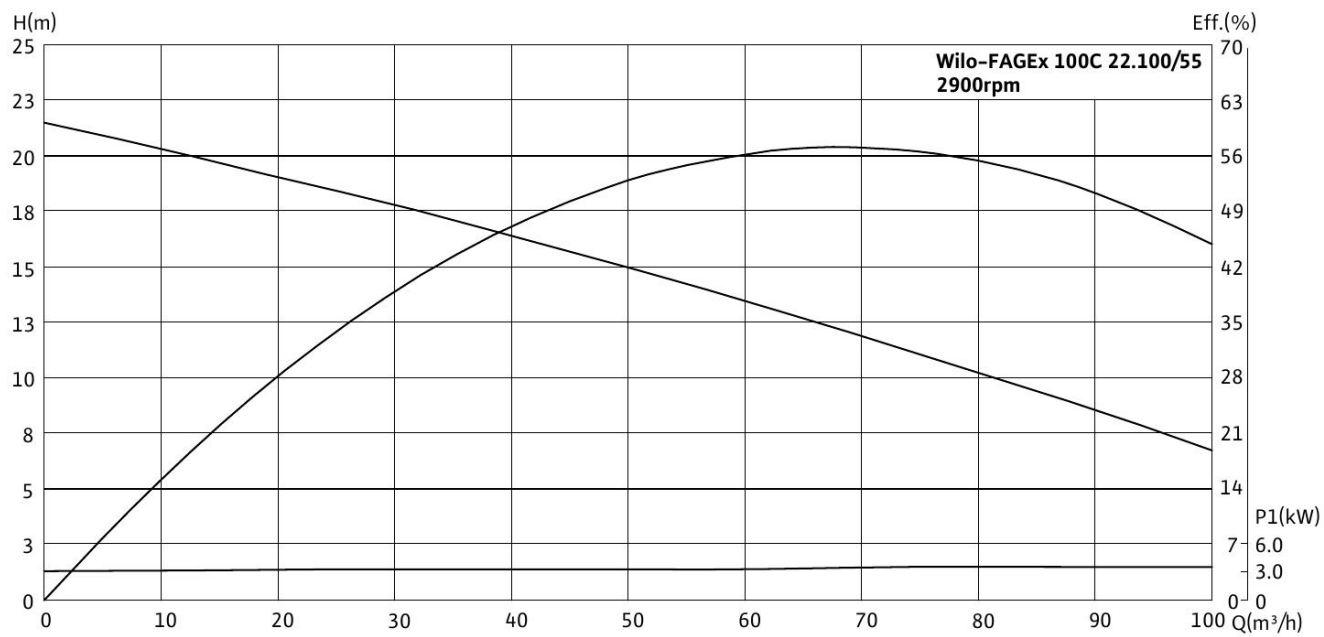
Wilo-FAGEx 100C 22.100/55
