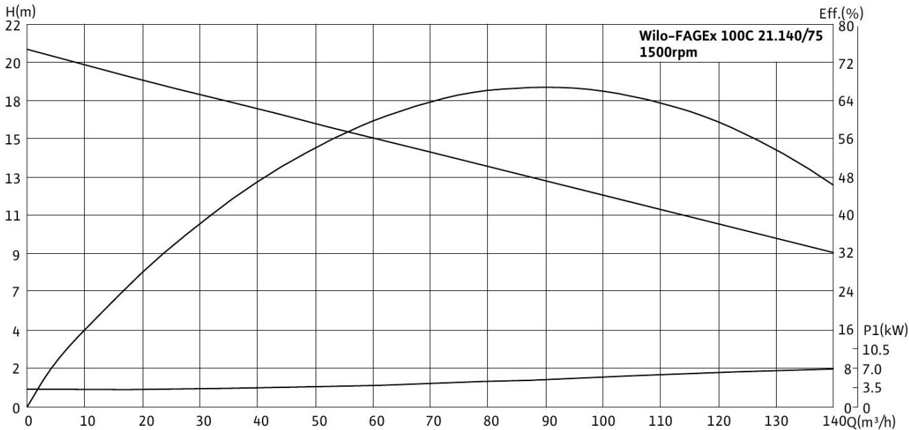
Wilo-FAGEx 100C 21.140/75
