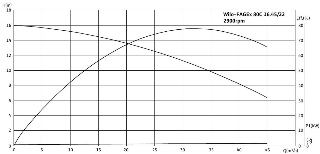
Wilo-FAGEx 80C 16.45/22
