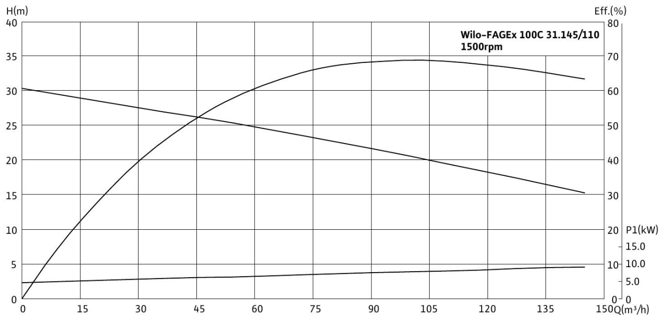
Wilo-FAGEx 100C 21.145/110
