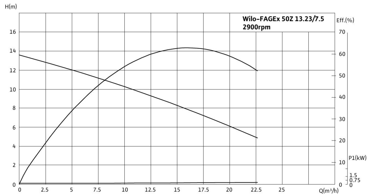
Wilo-FAGEx 50Z 13.23/7.5
