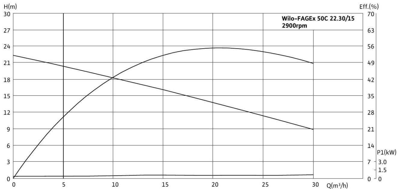
Wilo-FAGEx 50C 22.30/15
