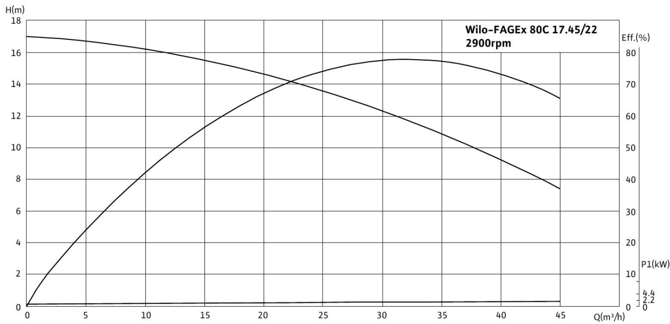
Wilo-FAGEx 80C 17.45/22
