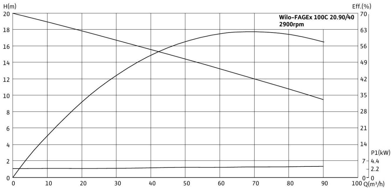
Wilo-FAGEx 100C 20.90/40
